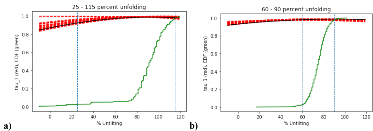
Figure S2. Results of bootstrap fold test for Packages 7 and 8. A bootstrap fold test after Tauxe & Watson (1994) was performed on site means obtained for Package 7 volcanics (a), Package 7 basalts (b) and Package 8 (c).
