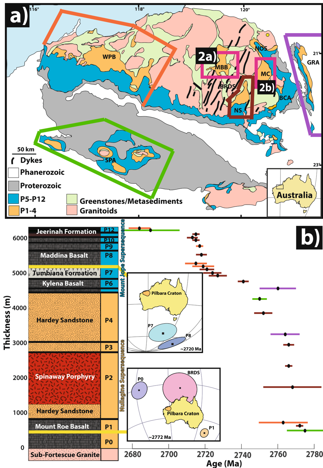
Fig. 1. Geologic context of the Fortescue Group as known prior to this study. The areal extent of the Fortescue Group is shown in (a) (after Blake et al., 2004), with abbreviations for the following regions: WPB – West Pilbara Basin; MBB – Marble Bar Basin; NS – Nullagine Syncline; MC – Meentheena Centrocline; GRA – Gregory Range Area; SPA – Southwest Pilbara Area; BCA – Boodalyeri Creek Area; NOS – North Oakover Syncline; BRDS – Black Range Dyke Swarm. Prior work on the stratigraphy (Thorne & Trendall, 2001), paleomagnetism (Evans et al., 2017; Strik, 2004), and geochronology (Blake et al., 2004, and references therein) is summarized in (b). The colored error bars for geochronology correspond to outcrop areas outlined in (a). Yellow lines indicate the two intervals of Fortescue stratigraphy discussed in this paper, between Packages 0 and 1 and Packages 7 and 8. (For interpretation of the references to color in this figure legend, the reader is referred to the web version of this article.)
