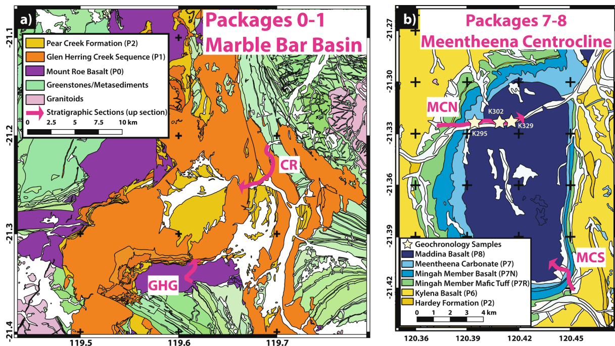
Fig. 2. Regional maps with stratigraphic sections. The Glen Herring Gorge (GHG) and Coongan River (CR) Package 0–1 stratigraphic sections were measured in the Marble Bar Basin, as seen on the geologic map in (a). Correlations of Package 0–1 stratigraphic units were guided by the radiometry mapping of Van Kranendonk et al. (2004). Package 7–8 stratigraphic sections were measured in the Meentheena Centrocline, with North (MCN) and South (MCS) sections highlighted in (b). Stratigraphic sections are highlighted in pink, with the arrowhead indicating the direction of upward in stratigraphy. (For interpretation of the references to color in this figure legend, the reader is referred to the web version of this article.)
