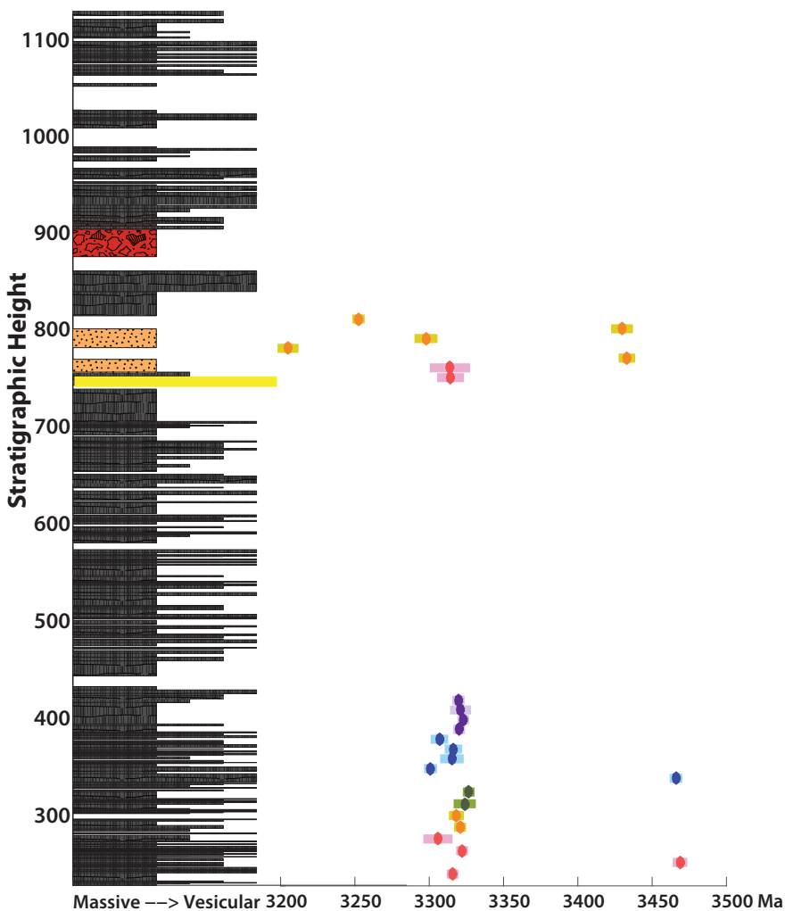
Figure S3. Glen Herring Gorge zircon dates. This figure shows the distribution of zircon dates obtained for geochronology samples collected from the Glen Herring Gorge section. These dates are similar to ages reported for the Duffer ( 3465 \pm 3 Ma) and Wyman Formations ( 3325 \pm 4 Ma), which outcrop near the basalt unconformity at GHG, as well as the Corunna Downs Granitoid Complex ( 3313 - 3300 Ma), located immediately southeast of the Marble Bar Basin (Australian Stratigraphic Units Database).
